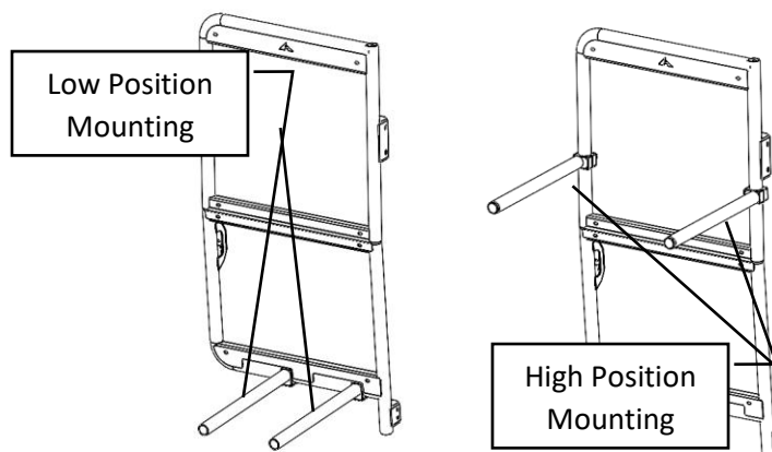
Figure 1: Configuration for Bolt-On Supports – Low (a) and High (b)
